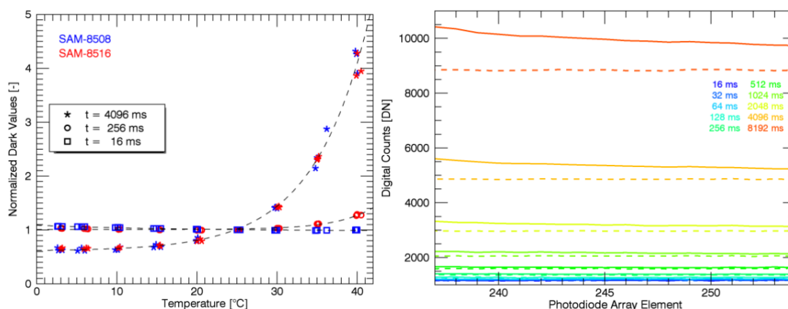
Figure 15. Dark signal values normalized at T=25\text{ °C} (left panel) determined for RAMSES SAM-8508 and RAMSES SAM-8516 with different integration times t , and counts (right panel) determined from the occulted elements of SAM-8516 with the entrance optics closed (dashed lined) and alternatively illuminated by an integrating sphere with saturation occurring for t > 256\text{ ms} (after Zibordi et al. 2017).
