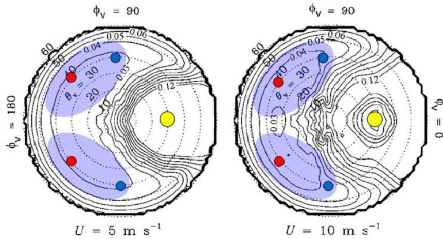
Figure 2. Distributions of \rho -factors as a function of the viewing and relative azimuth angles for wind speeds of 5 and 10 m s^{-1} , and sun zenith of 30^\circ (adapted from Mobley 1999). The yellow filled circle mirrors the sun position. The shadowed light-blue areas highlight viewing geometries most suitable for above-water radiometry. The blue and red filled circles indicate the L_T viewing geometries relying on \phi = 135^\circ and \phi = 90^\circ , respectively.
