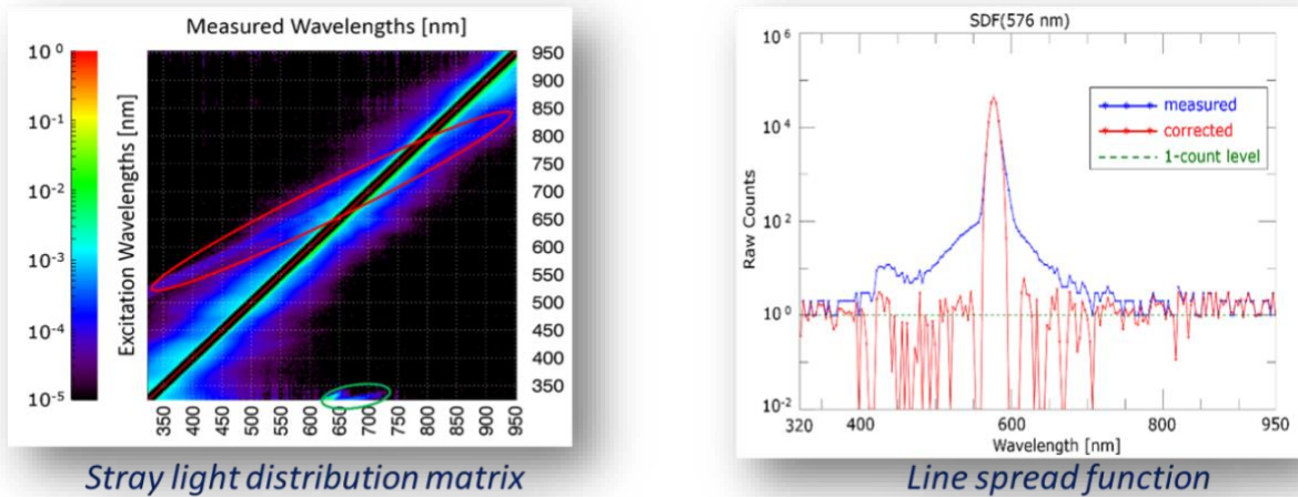
Figure 9. Stray light distribution matrix ( left panel ) for the hyperspectral radiometer SAM-8346 and application of the stray light correction matrix to a monochromatic signal at 576 nm ( right panel ). In the left panel the measurement and excitation wavelengths are on the x and y axes in units of nm, respectively. The values of the matrix coefficients, in normalized (raw) counts, are displayed in log-scale. The green and red ellipses highlight spectrally extended stray light perturbations. The black straight lines near the diagonal identify the in-band response regions. In the right panel the measured and the corrected signals are shown in blue and red, respectively. The 1-count level is indicated by the dashed line (reprinted from Talone et al. 2016). It is likely that instrument batches manufactured applying the same design and optical components, exhibit very similar stray light perturbations. Once verified, this would allow to confidently apply the same stray light correction procedure to all the radiometers from the batch.
