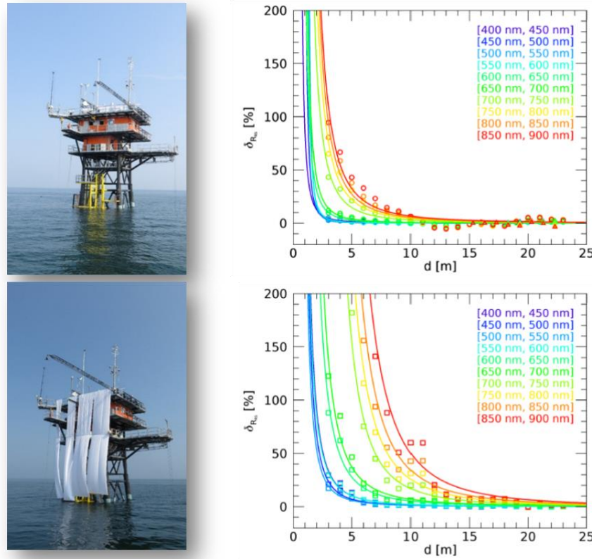
Figure 13. Spectral changes \delta_{R_{RS}}(l) affecting R_{RS}(l) as a function of the distance from the superstructure for actual measurement conditions ( i.e. , low reflectance) in the upper panels and additionally, for measurement conditions worsened by the increased reflectance of the superstructure ( i.e. , high reflectance) in the lower panels (after Talone and Zibordi 2019). The superstructure height h is 17 m. It is assumed that \delta_{R_{RS}}(l) = 0 in the far field ( i.e. , well away from the superstructure): this is tentatively fulfilled with d \sim 17 m for the low reflectance case and with d \sim 25 m for the high reflectance case.
