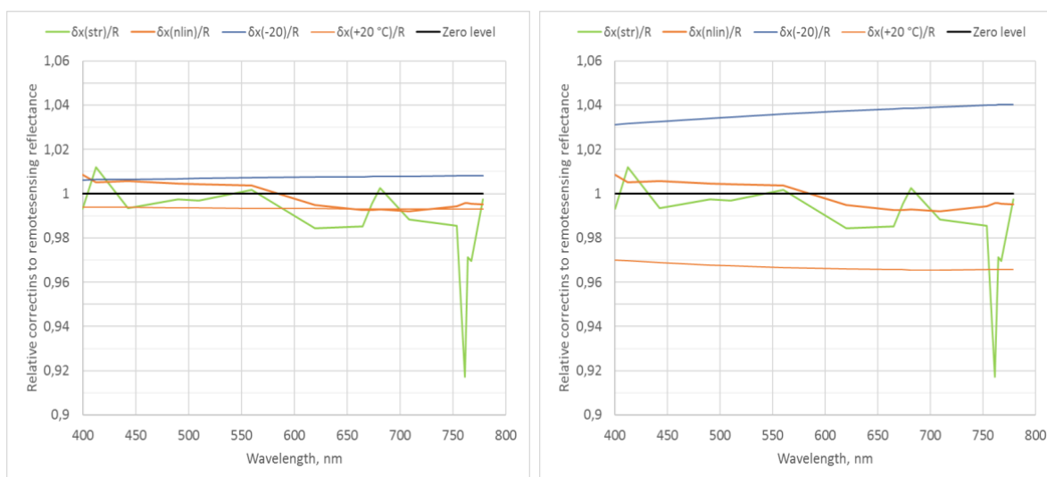
Figure 1-2. Simulation of joint relative effects for the three-radiometer's system due to straylight, nonlinearity and temperature difference during calibration and later use. Left: System with three RAMSES sensors; Right: system with three HyperOCR sensors.
