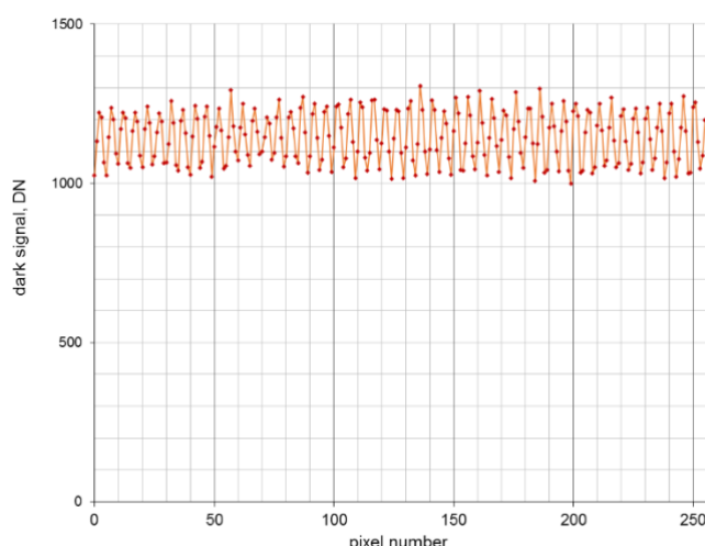
Figure 4-7. Oscillations of the dark signal imply the need for repair.
