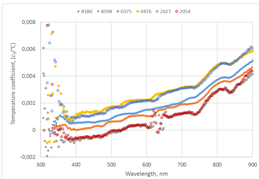
Figure 4-8. Thermal coefficients of two RAMSES and four HyperOCR sensors after correction for non-linearity.
