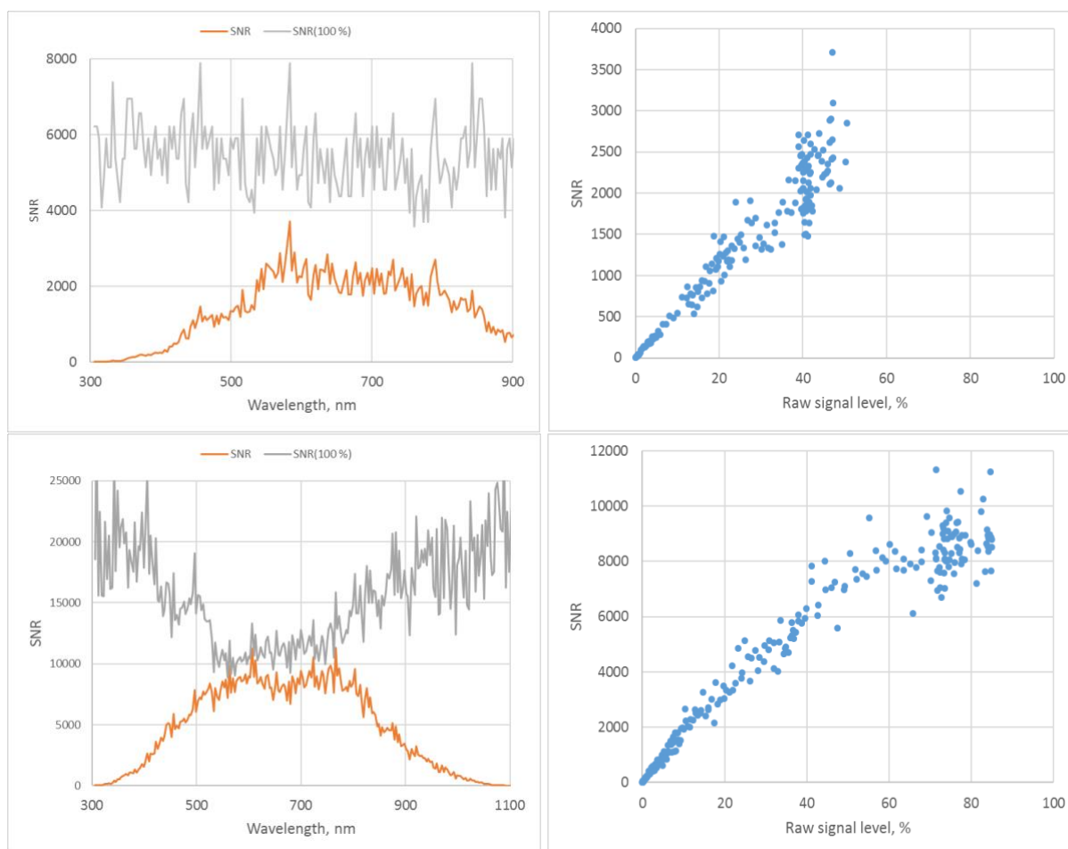
Figure 4-11. Signal-to-noise ratio (left) and SNR as a function of raw signal (right). HyperOCR radiometer (upper part) and RAMSES (lower part).
