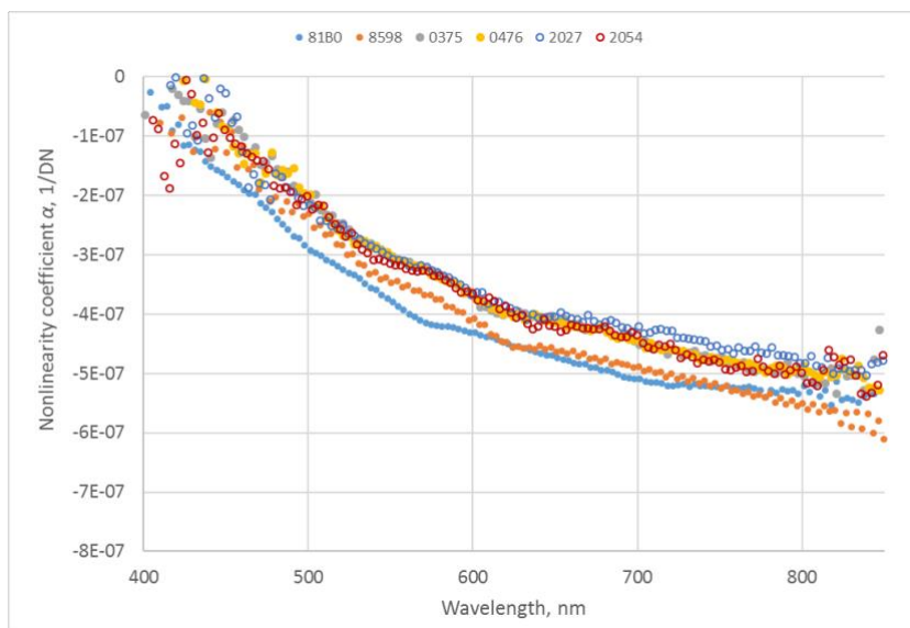
Figure 4-5. Averaged non-linearity coefficient \alpha of two RAMSES and four HyperOCR sensors.
