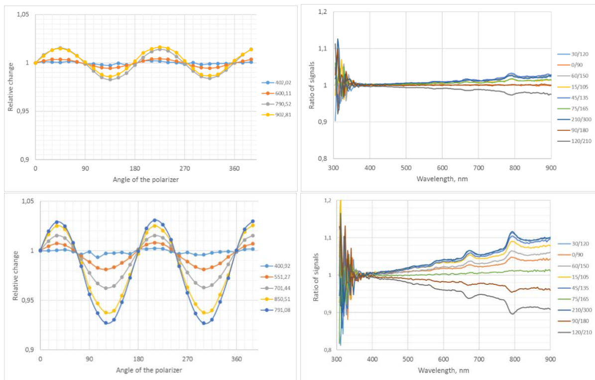
Figure 4-10. Relative polarisation effect as a function of angle and wavelength. RAMSES radiance sensor (upper part) and HyperOCR radiance sensor (lower part).
