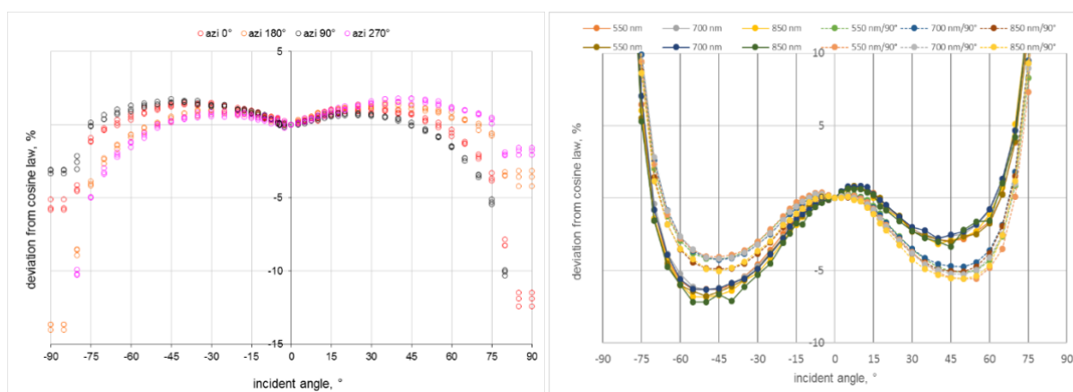
Figure 4-2. Angular response of HyperOCR (left) and RAMSES (right) irradiance sensors.
