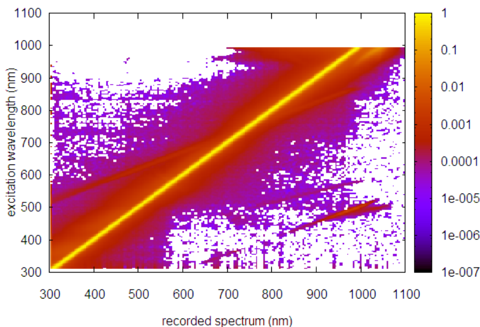
Figure 4-1. Stray light matrix of a RAMSES sensor. Diagonal values of the SLM are normalised to 1.
