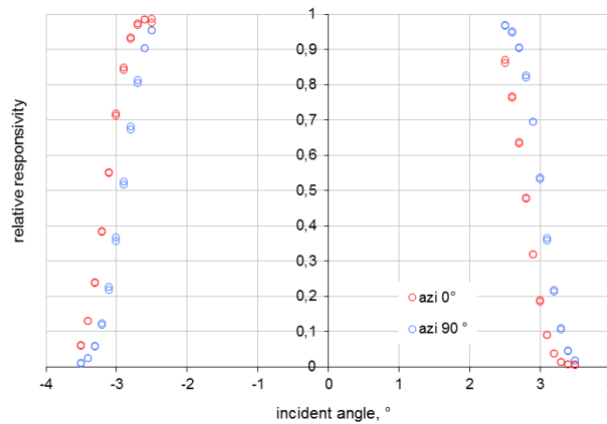
Figure 4-4. FOV of above-water HyperOCR radiance sensors.
