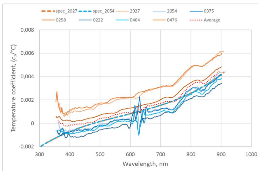
Figure 4-9. Thermal coefficients of seven HyperOCR sensors and thermal responsivity data for two sensors calculated according to the guidance of the Seabird's Sensor System Group.
