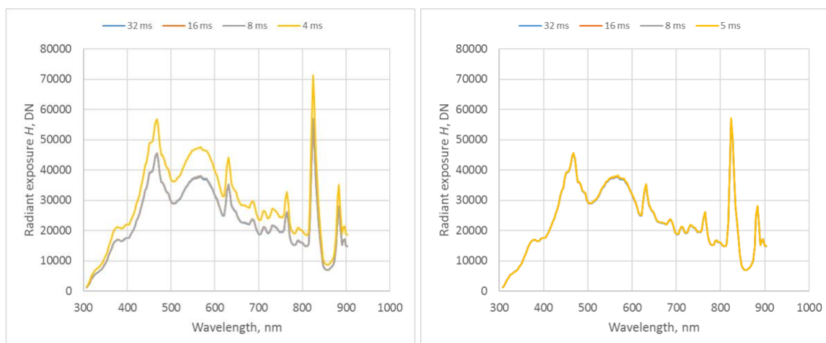
Figure 4-6. Xe-lamp spectra measured by using four integration times and normalised to the same radiant exposure. Left: for the value set to 4 ms large bias is evident; right: after applying the actual value of 5 ms normal agreement is achieved.
