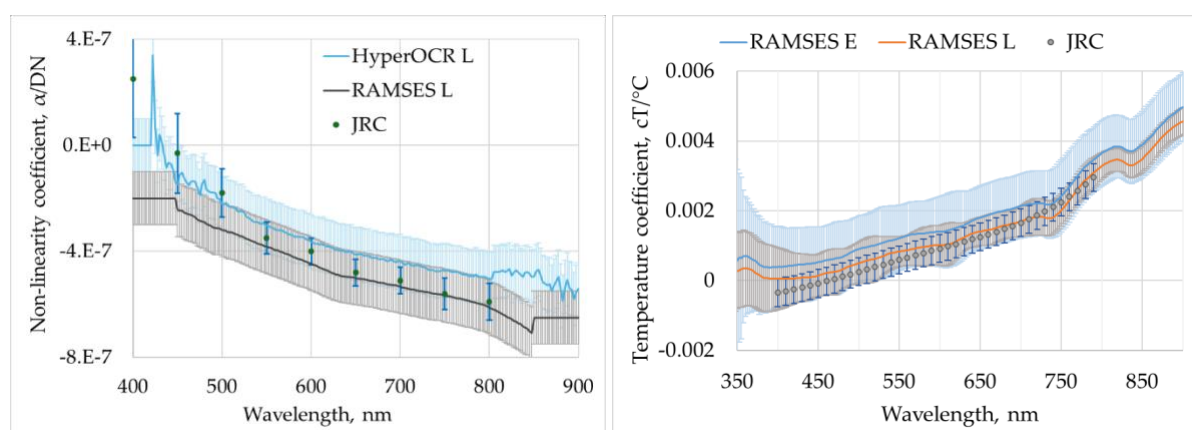
Figure 6-1. Class-specific characteristics with expanded uncertainty. Left: Non-linearity coefficients. Right: Temperature coefficients.
