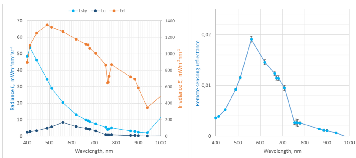
Figure 1-1. Spectra measured with three radiometers (left) for determination of remote sensing reflectance (right) convoluted to OLCI bands. With uncertainty bars, combined expanded uncertainty is shown.
