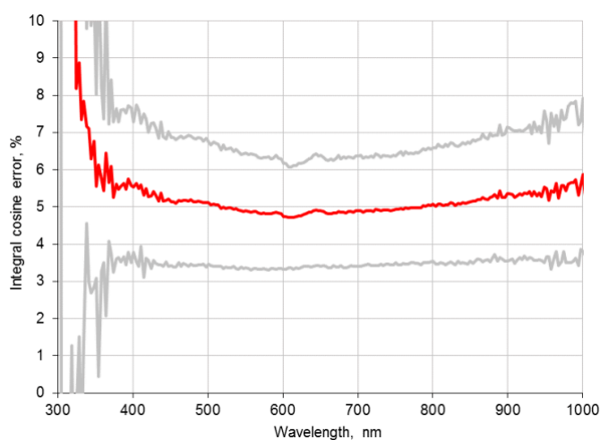
Figure 4-3. Integral cosine error with expanded uncertainty bars of a RAMSES irradiance sensor.
